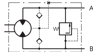
EPMM Series with Integrated Internal Crossover Relief Valve B → A, Δp = 100 bar (50 bar)
