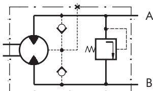
EPMM Series with Integrated Internal Crossover Relief Valve A → B, Δp = 100 bar (50 bar)
